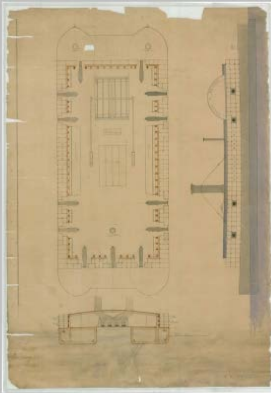
Plan of Defence for Wrecking Boat, Submarine No 7 - USS Benton--746.jpg 4.26 MB
